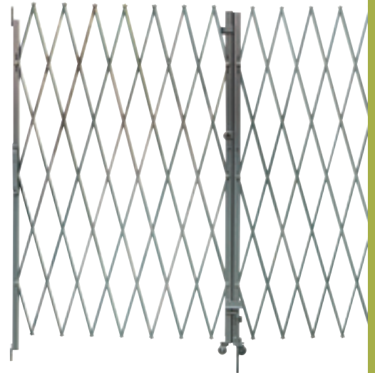
VALUE BRAND Steel Folding Gates Steel folding gates feature 15-gauge U-channels riveted back-to-back and are equipped with self-securing center drop-in pin. 12-gauge steel vertical gate rails. Galvanized finish. Universal mounting on face or in casing. brackets, bearing washers, casters and lock lugs included. Padlocks NOT included.
