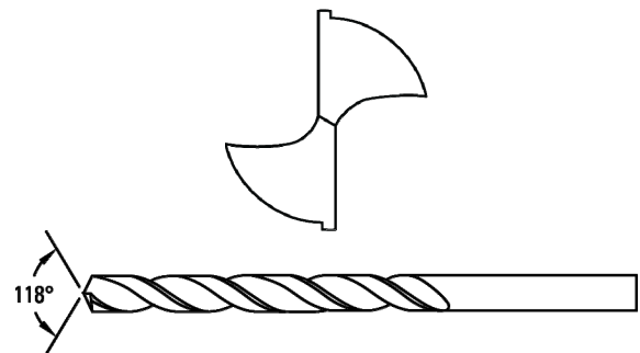
118° General-Purpose Point
